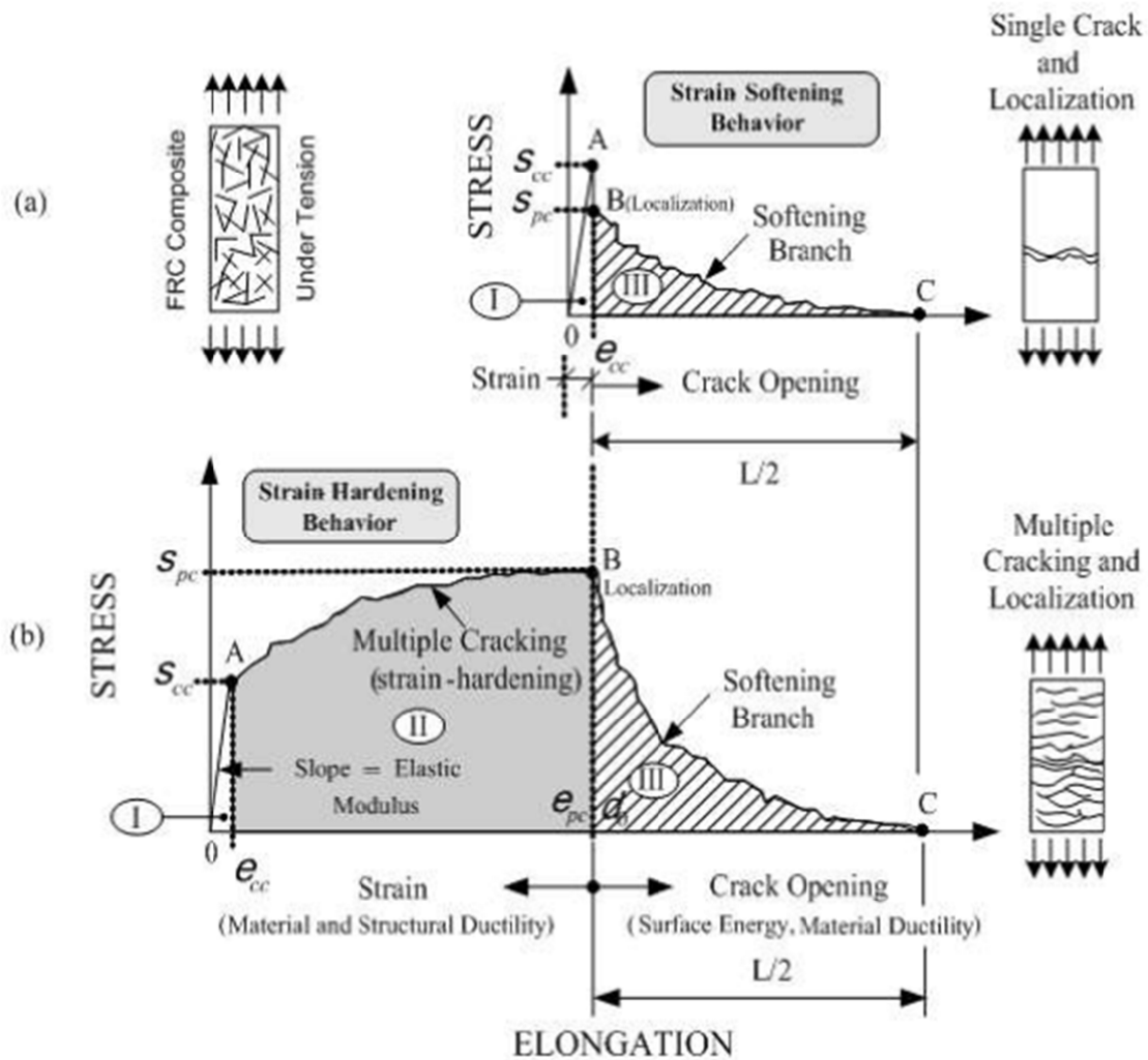
Figure 2.4: Principal cracking behaviour when the fibre concrete specimen are subjected to stress–elongation. (a) Strain-softening behaviour. (b) Strain-hardening behaviour (HPCFRCC). (Naaman, 2007)
