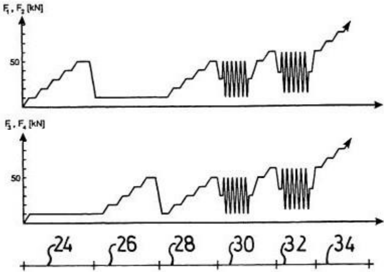
Figure 3.10: Loading scheme. The picture illustrates course of various loads applied to the inventions and the fixed structure. (Thoof et al., 2001)
