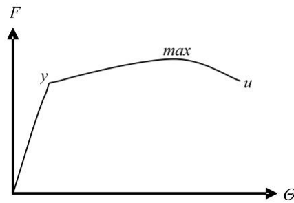
Figure 3.2: Definition of significant load steps, from (Schumacher et al., 2009).
